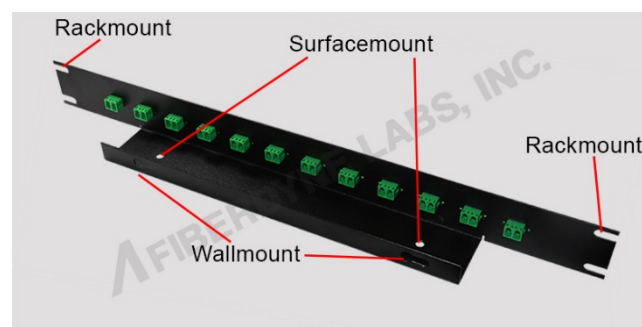
12 Port Panel (Back)
