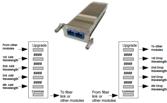
Multiplexer (Mux)
