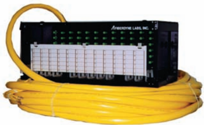
RTP-072 with 72 Fiber Pigtail
